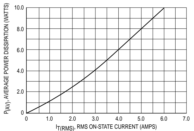
FIGURE 2 — POWER DISSIPATION
