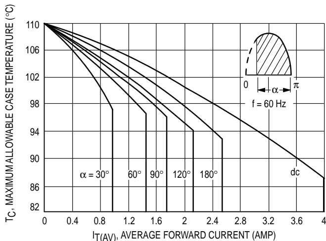
Figure 2. Maximum Case Temperature
