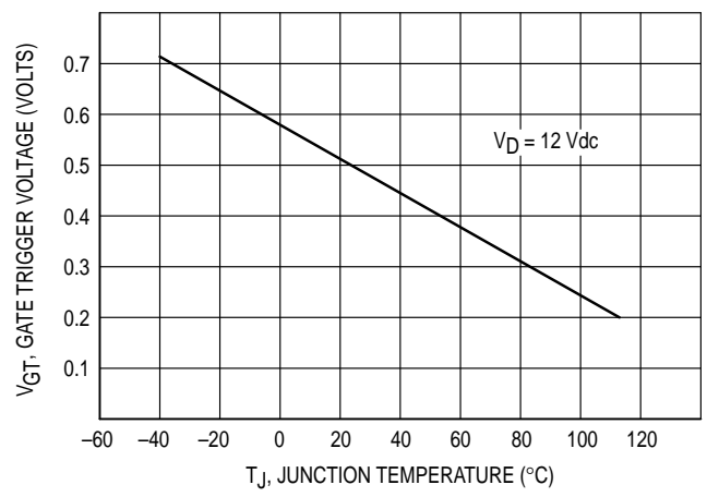
FIGURE 4 – GATE VOLTAGE
