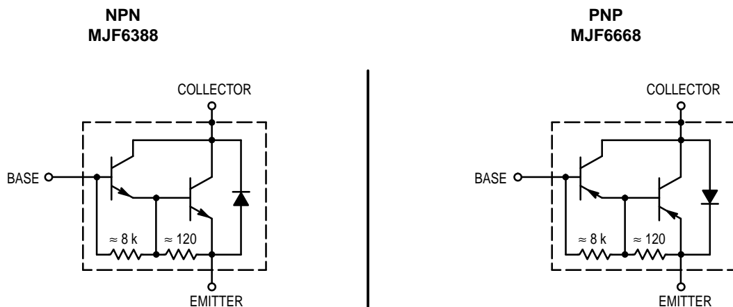
Figure 1. Darlington Schematic
