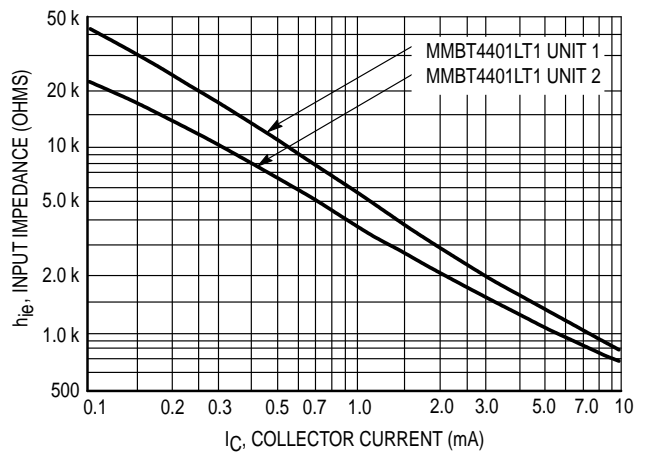
Figure 12. Input Impedance
