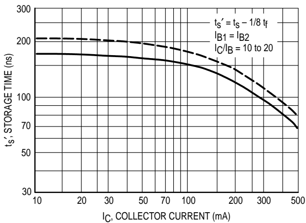
Figure 7. Storage Time
