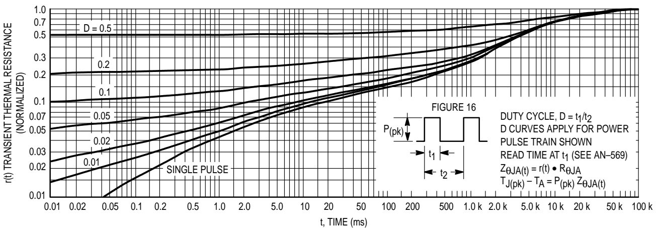
Figure 14. Thermal Response
