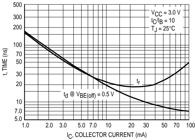
Figure 10. Turn-On Time
