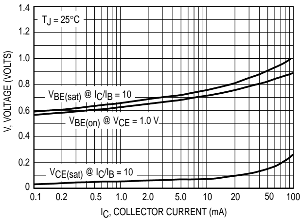
Figure 8. "On" Voltages
