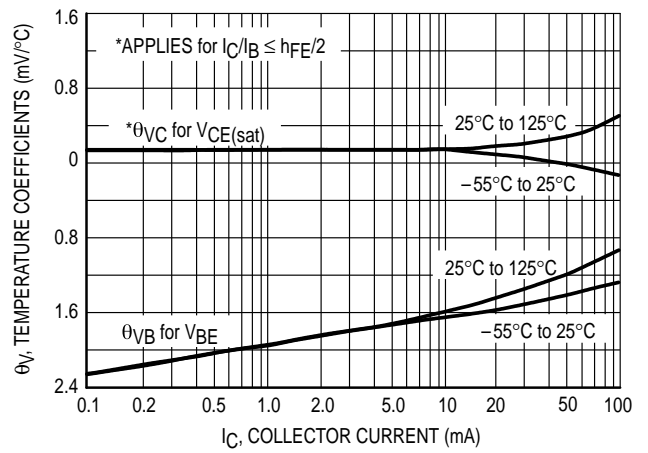
Figure 9. Temperature Coefficients
