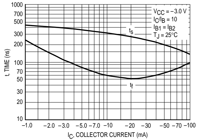
Figure 11. Turn-Off Time
