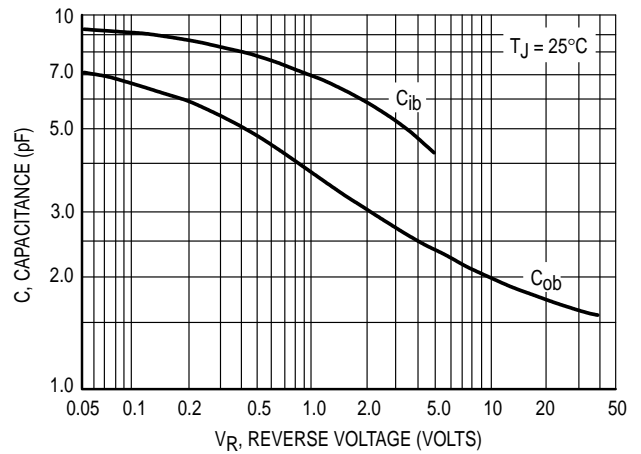
Figure 13. Capacitance
