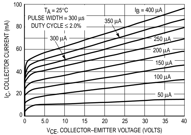
Figure 7. Collector Characteristics
