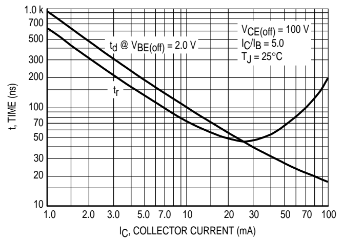
Figure 6. Turn-On Time
