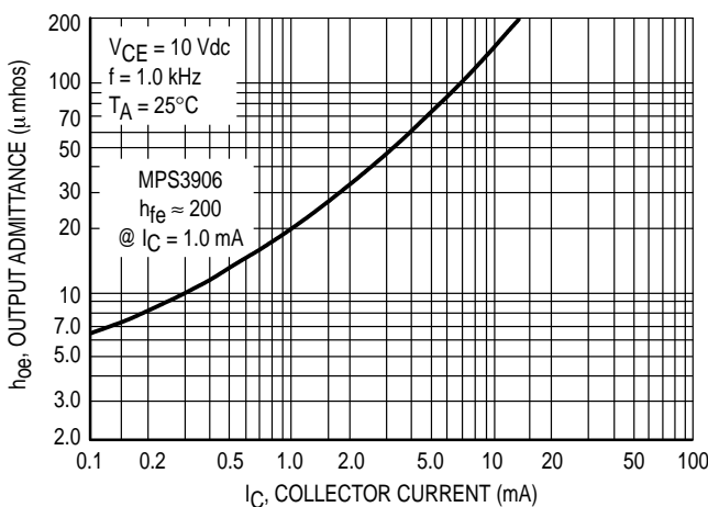
Figure 16. Output Admittance
