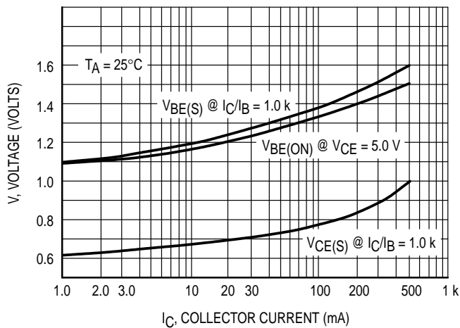
Figure 2. "ON" Voltages
