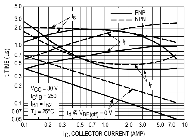
Figure 3. Switching Times
