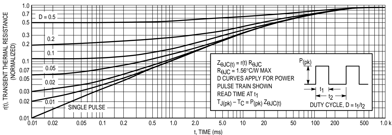
Figure 4. Thermal Response
