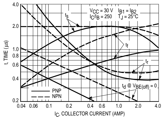
Figure 3. Switching Times
