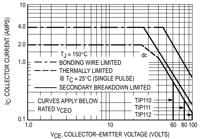
Figure 6. TIP110, 111, 112
