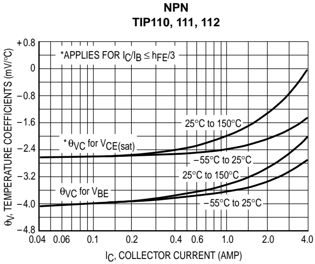
Figure 11. Temperature Coefficients
