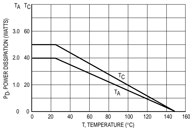
Figure 1. Power Derating
