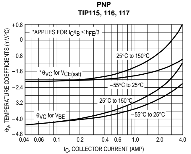
Figure 11. Temperature Coefficients
