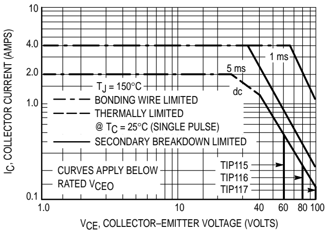
Figure 5. TIP115, 116, 117
