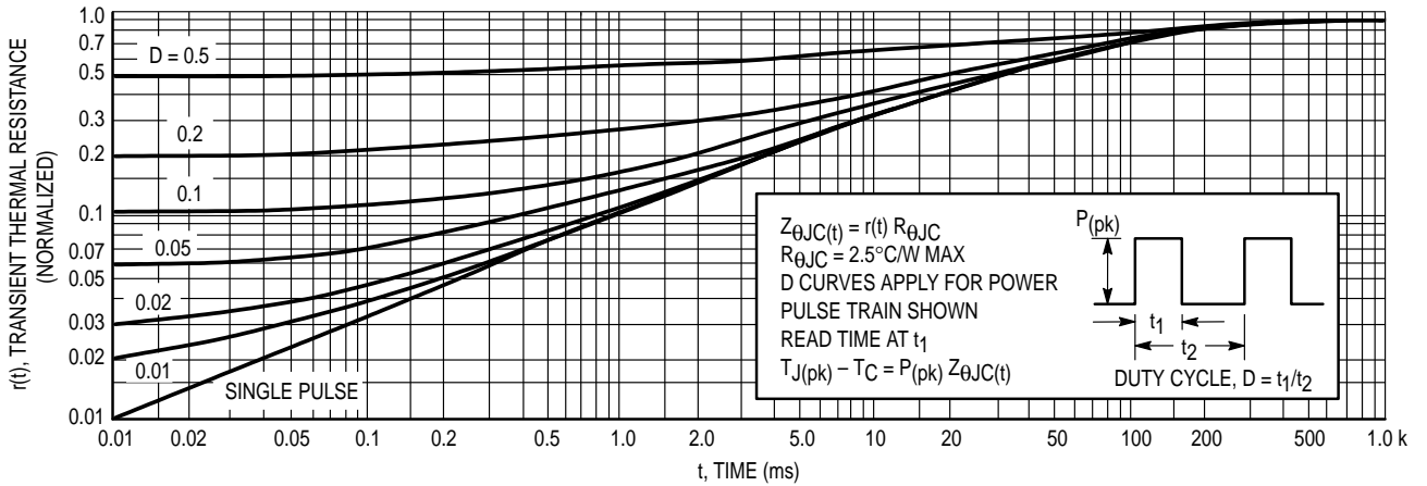
Figure 4. Thermal Response
