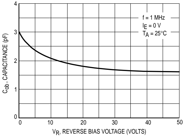
Figure 9. Output Capacitance
