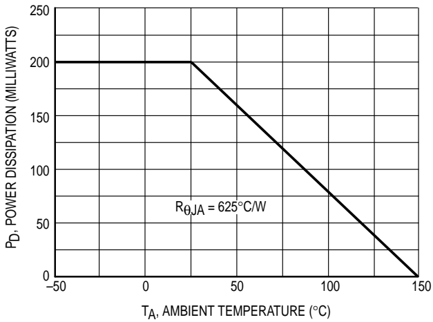
Figure 1. Derating Curve
