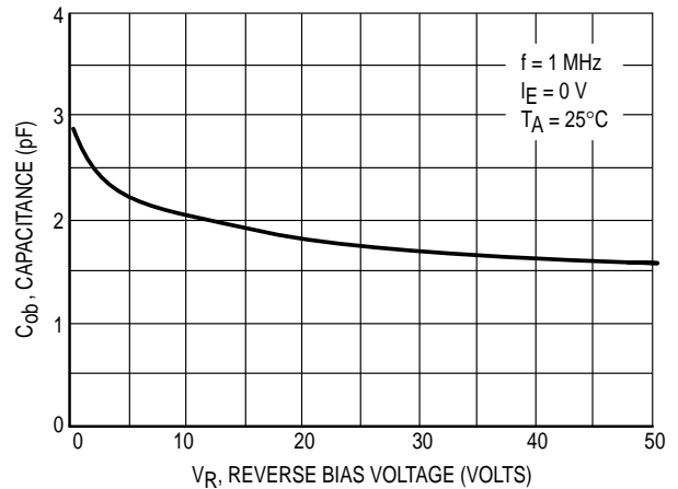
Figure 4. Output Capacitance
