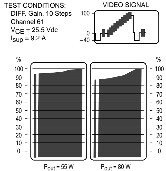
Figure 5. Differential Gain
