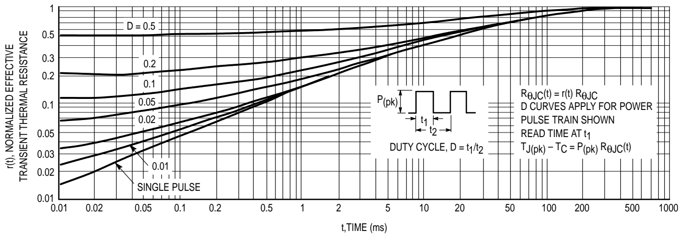
Figure 13. Thermal Response
