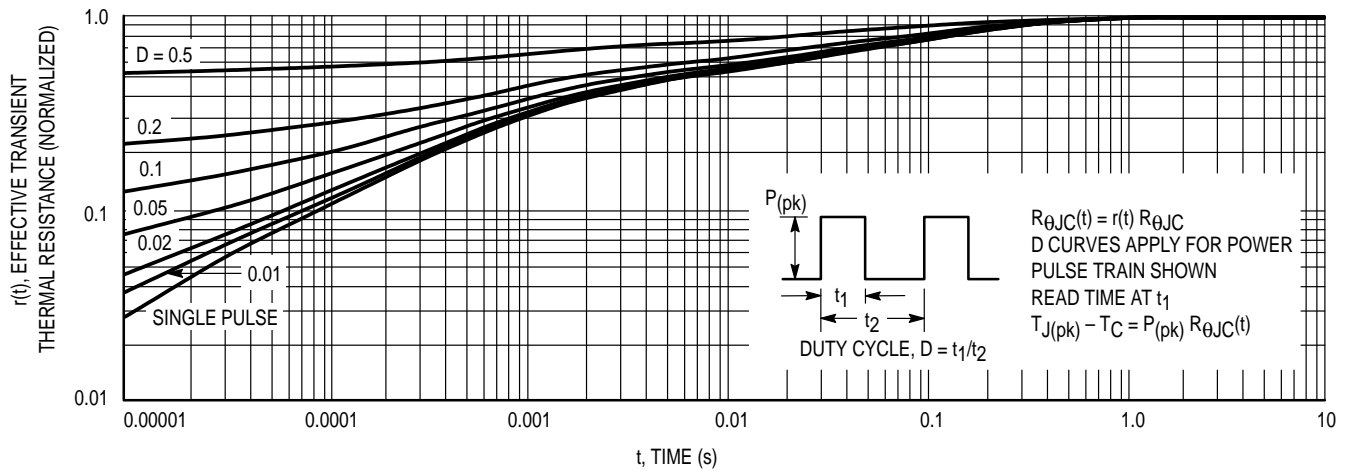
Figure 14. Thermal Response
