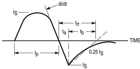
Figure 16. Diode Reverse Recovery Waveform
