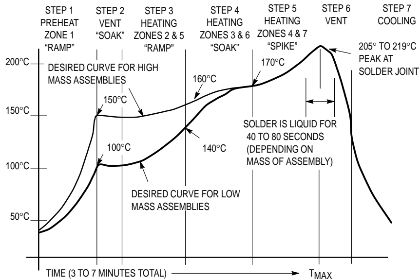
Figure 17. Typical Solder Heating Profile
