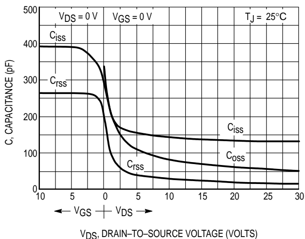
Figure 9. Capacitance Variation
