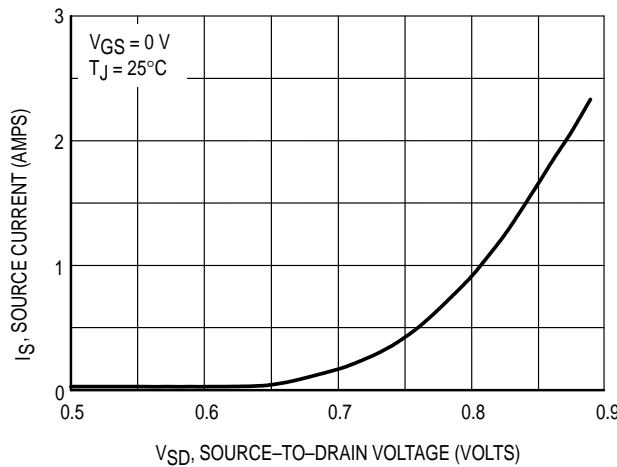
Figure 12. Diode Forward Voltage versus Current
