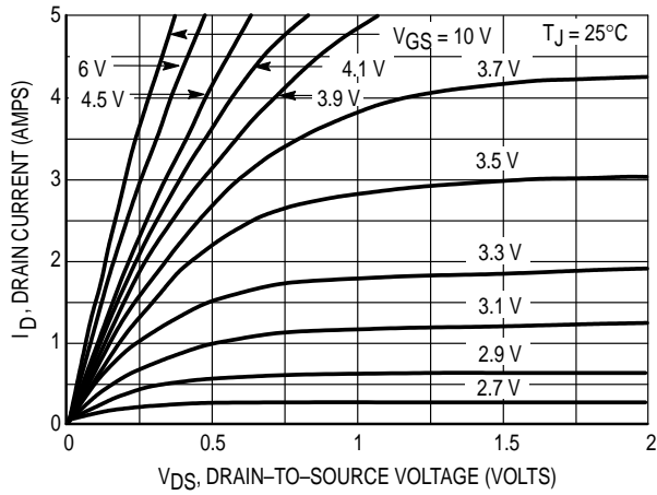
Figure 3. On-Region Characteristics
