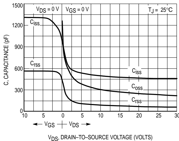
Figure 9. Capacitance Variation
