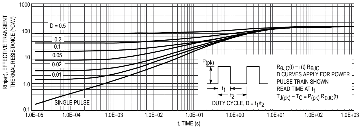
Figure 16. Thermal Response
