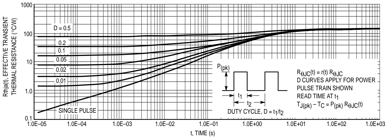
Figure 15. Thermal Response
