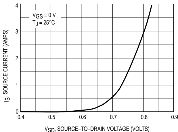
Figure 12. Diode Forward Voltage versus Current
