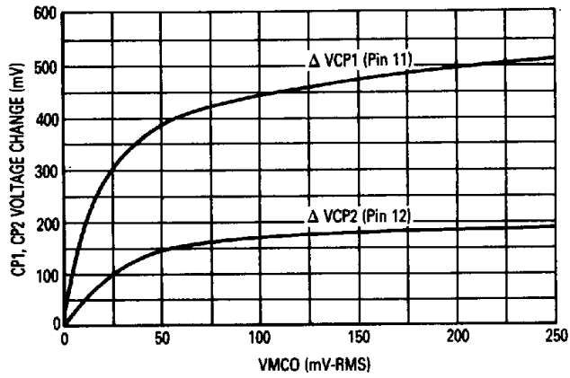
FIGURE 11 — TRANSMIT DETECTOR OPERATION
