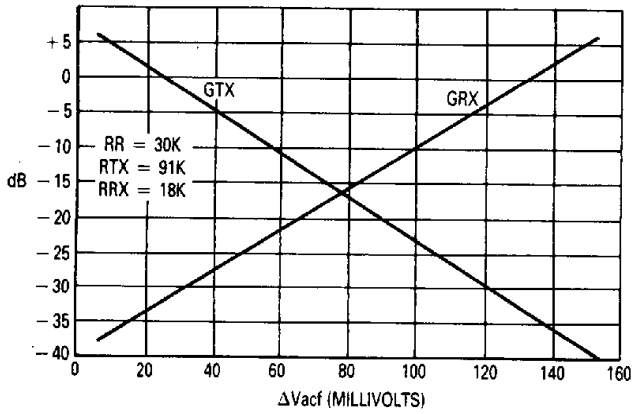
FIGURE 6 — ATTENUATOR GAIN versus ΔVacf
