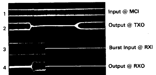
FIGURE 17 — IDLE-RECEIVE SWITCHING
