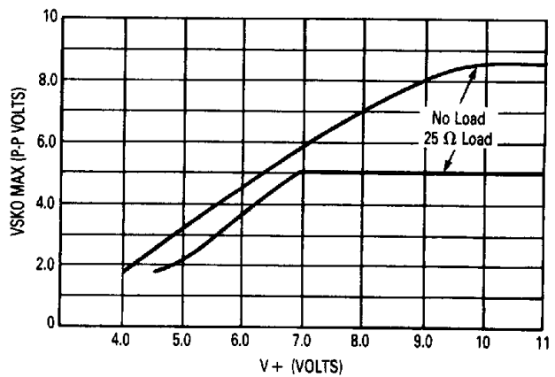
FIGURE 9 — SPEAKER AMP OUTPUT versus SUPPLY VOLTAGE
