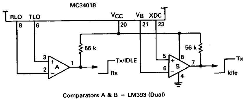
FIGURE 20 — DIGITAL TRANSMIT/IDLE/RECEIVE INDICATION
