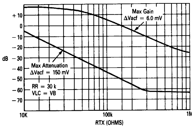
FIGURE 2 — TRANSMIT ATTENUATOR versus RTX
