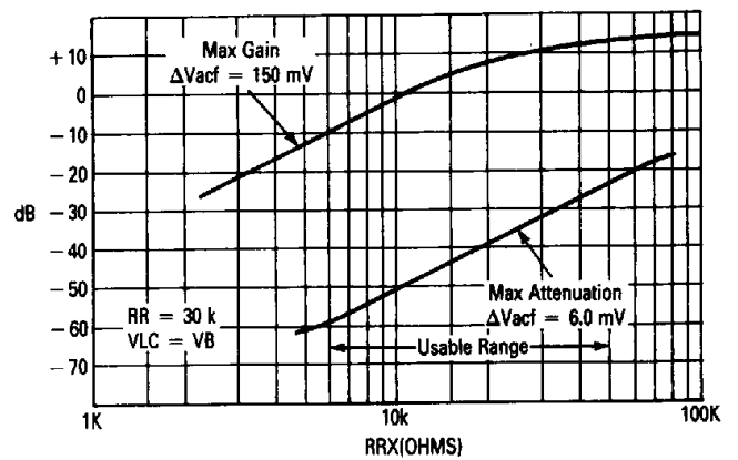
FIGURE 3 — RECEIVE ATTENUATOR versus RRX
