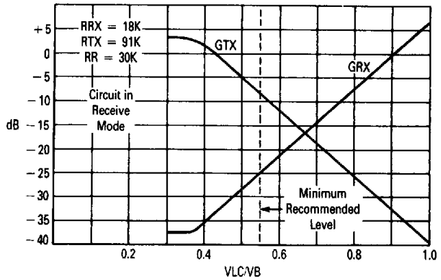
FIGURE 5 — ATTENUATOR GAIN versus VLC
