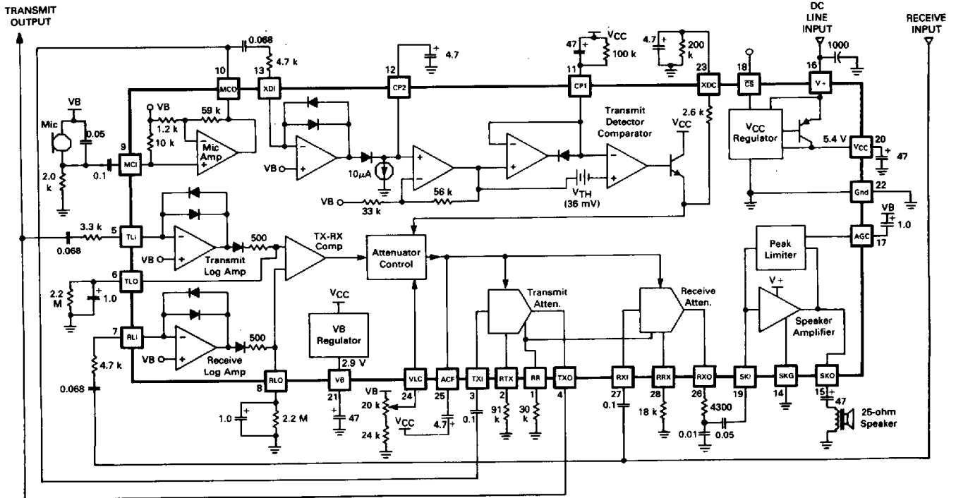
FIGURE 1 — TEST CIRCUIT
