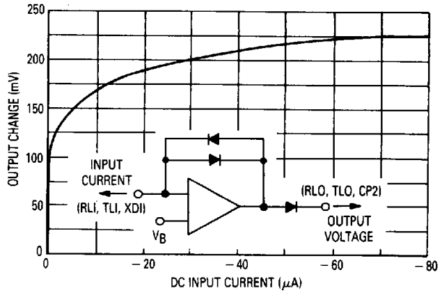
FIGURE 7 — LOG AMP TRANSFER CHARACTERISTICS
