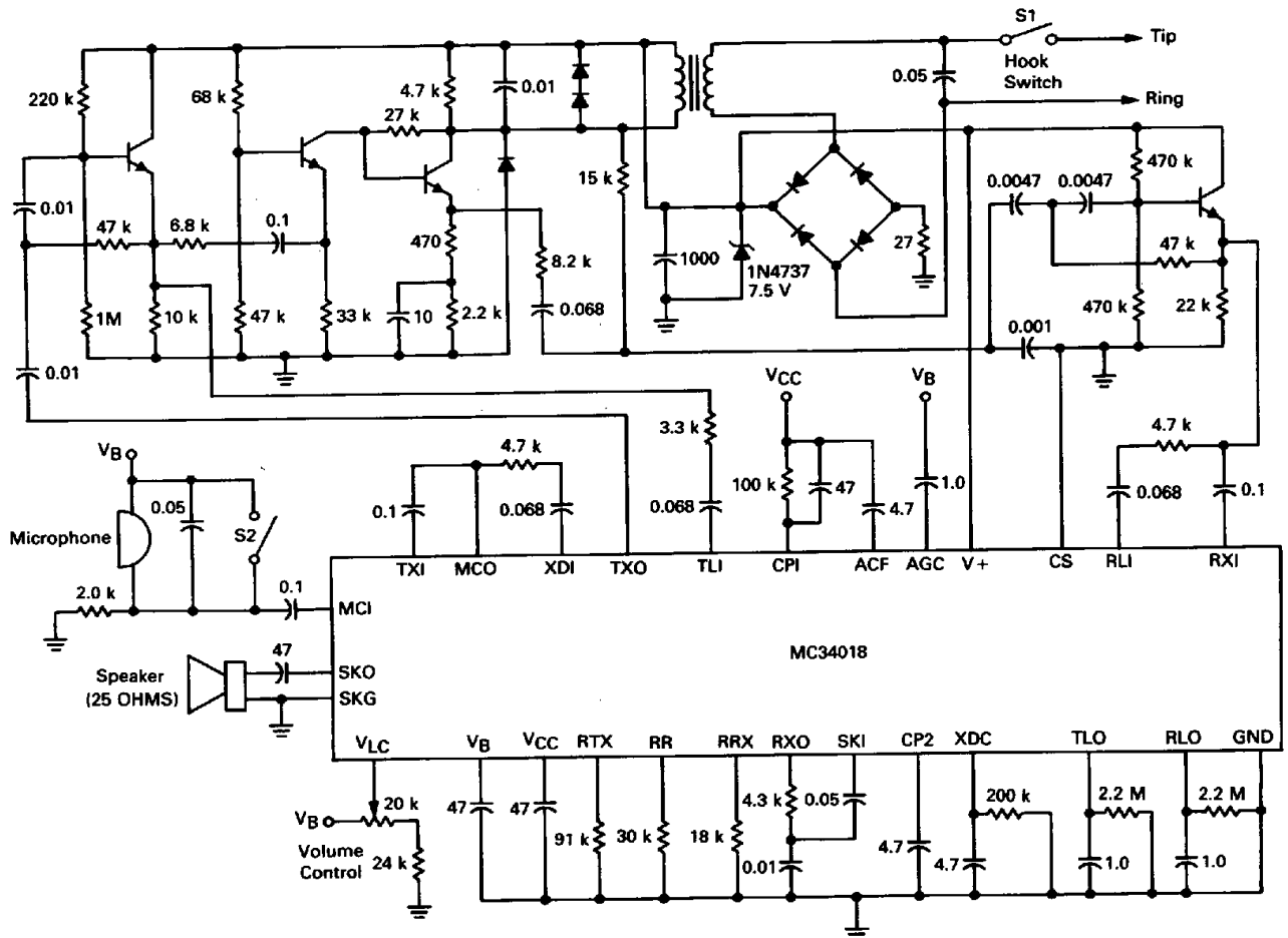
FIGURE 19 — BASIC LINE POWERED SPEAKERPHONE
