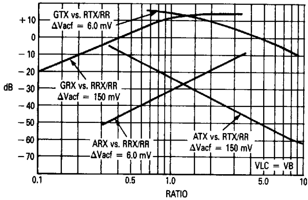
FIGURE 4 — GAIN AND ATTENUATION versus RESISTOR RATIOS
