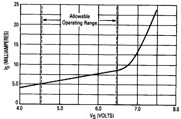
FIGURE 15 — SUPPLY CURRENT versus SUPPLY VOLTAGE (SEE FIGURE 14)
