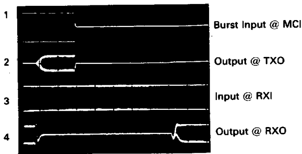
FIGURE 16 — TRANSMIT-RECEIVE SWITCHING
