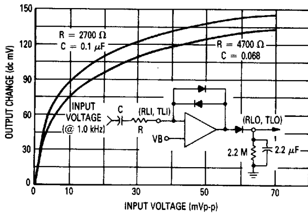
FIGURE 8 — LOG AMP TRANSFER CHARACTERISTICS
