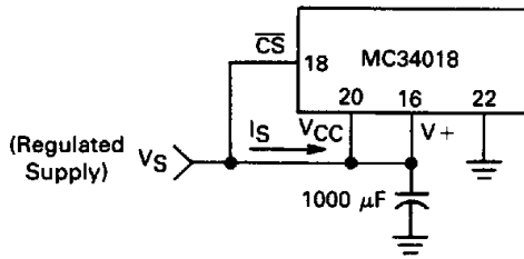
FIGURE 14 — ALTERNATE POWER SUPPLY CONFIGURATION
