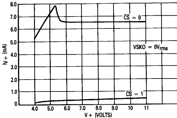
FIGURE 12 — SUPPLY CURRENT versus SUPPLY VOLTAGE
