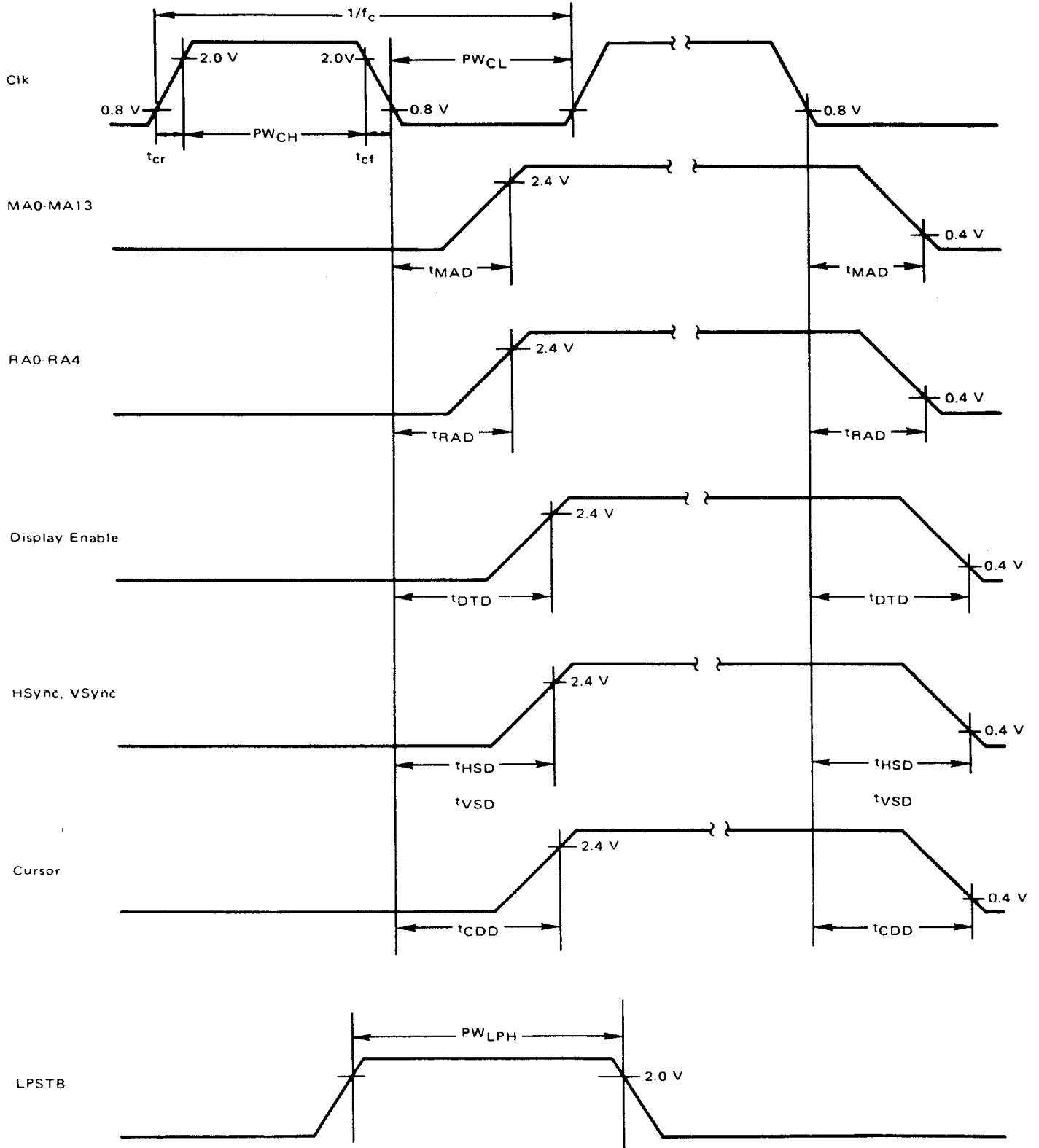
FIGURE 3 - CRTIC TIMING CHART
