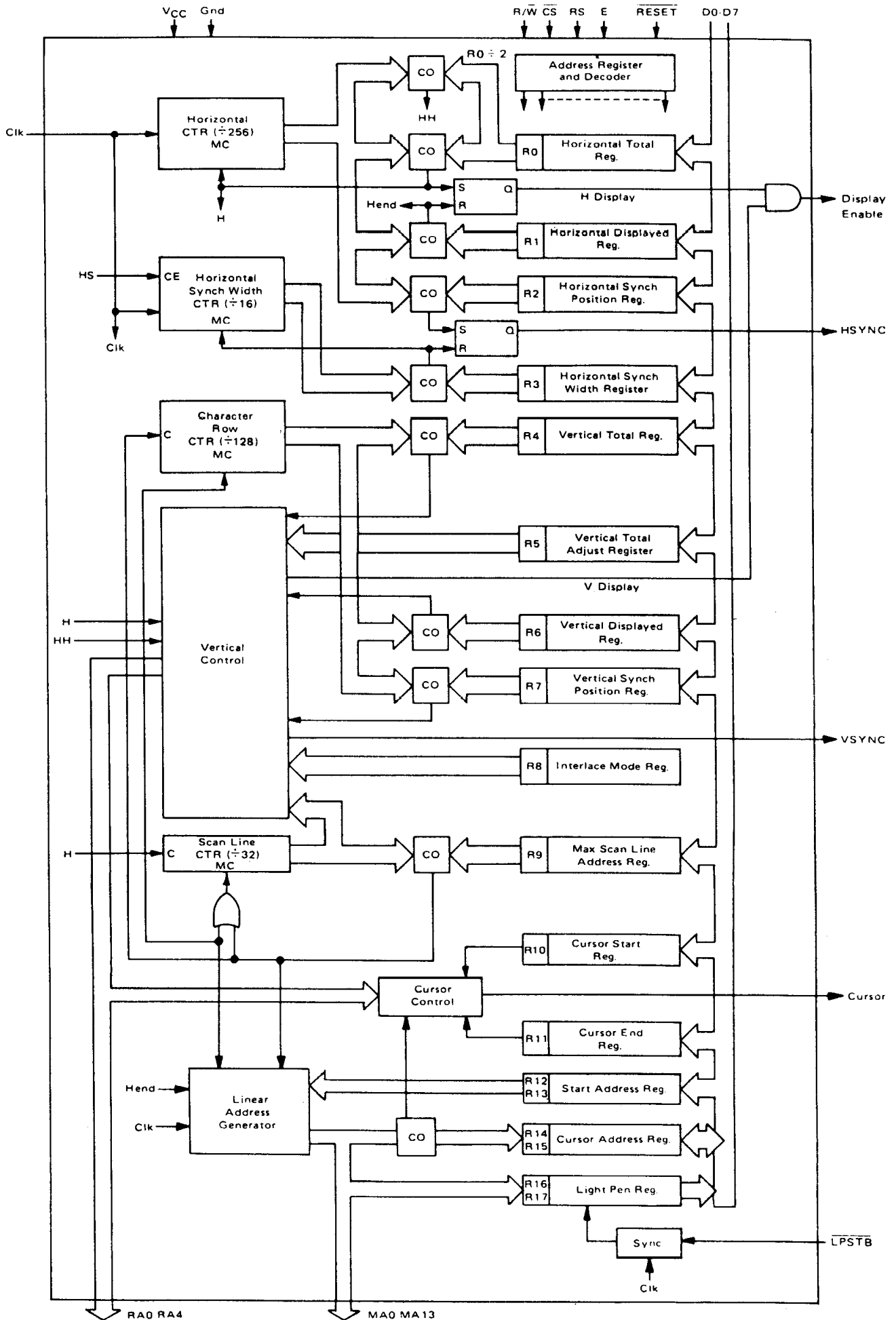
FIGURE 8 - CRTC FUNCTIONAL BLOCK DIAGRAM
