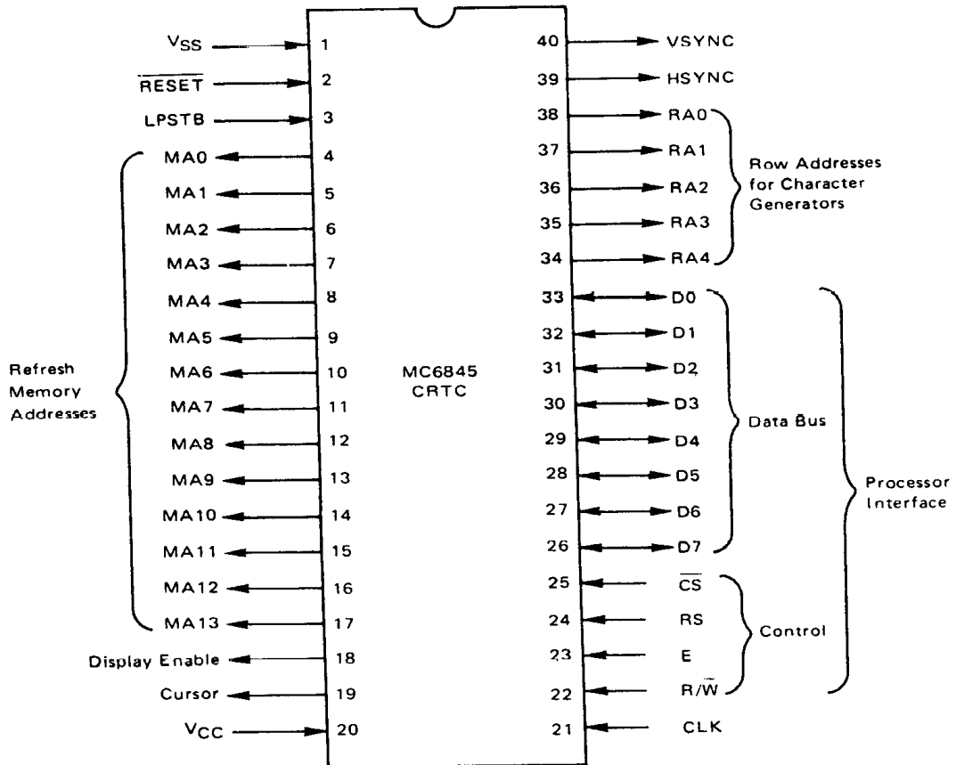
FIGURE 7 – PIN ASSIGNMENT
