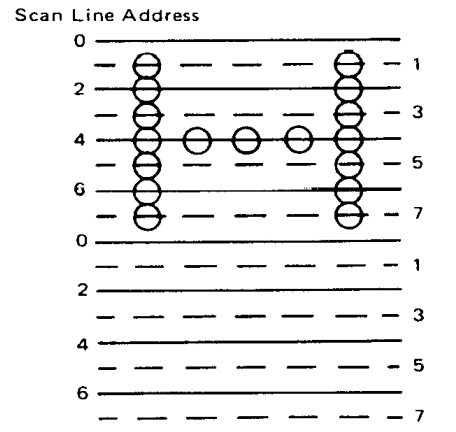
Interlace Sync and Video
