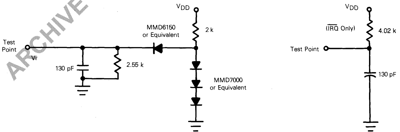
FIGURE 6 — TTL EQUIVALENT TEST LOAD
