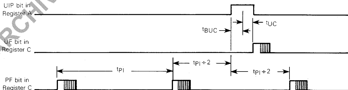
FIGURE 15 — UPDATE-ENDED AND PERIODIC INTERRUPT RELATIONSHIP
