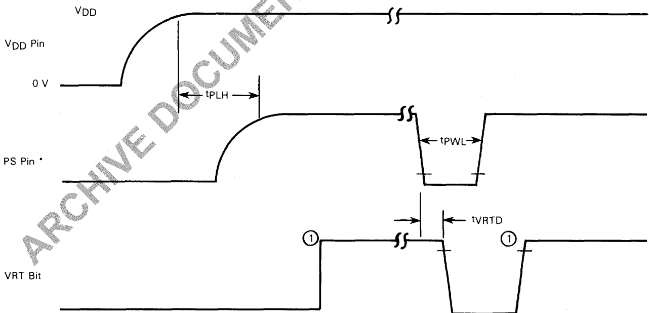
FIGURE 8 — CONDITIONS THAT CLEAR VRT BIT
