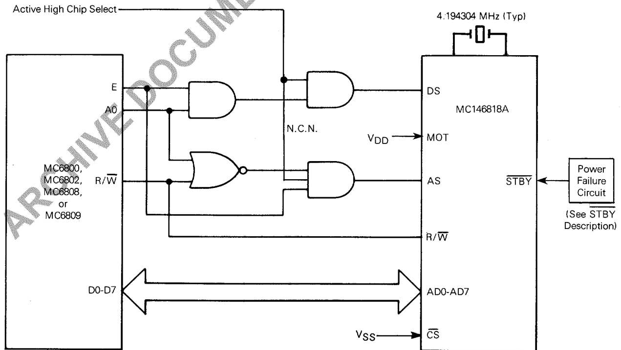
FIGURE 20 — MC146818A INTERFACED WITH MOTOROLA PROCESSORS
