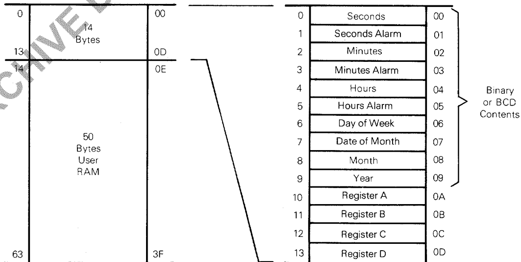
FIGURE 14 — ADDRESS MAP
