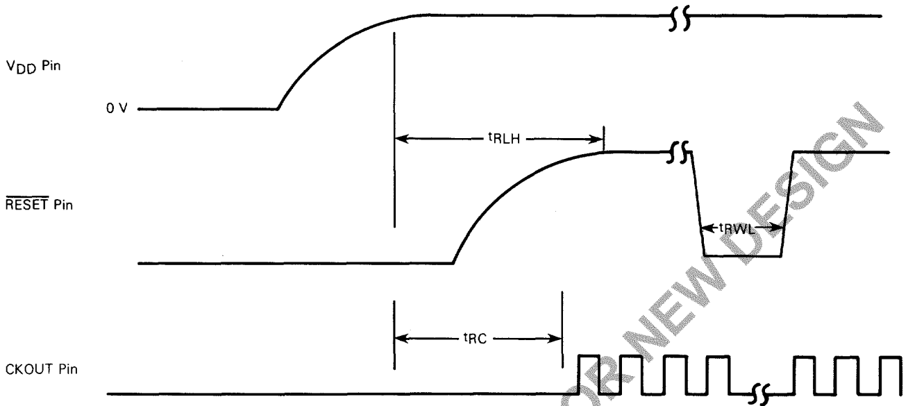
FIGURE 7 — POWER-UP
