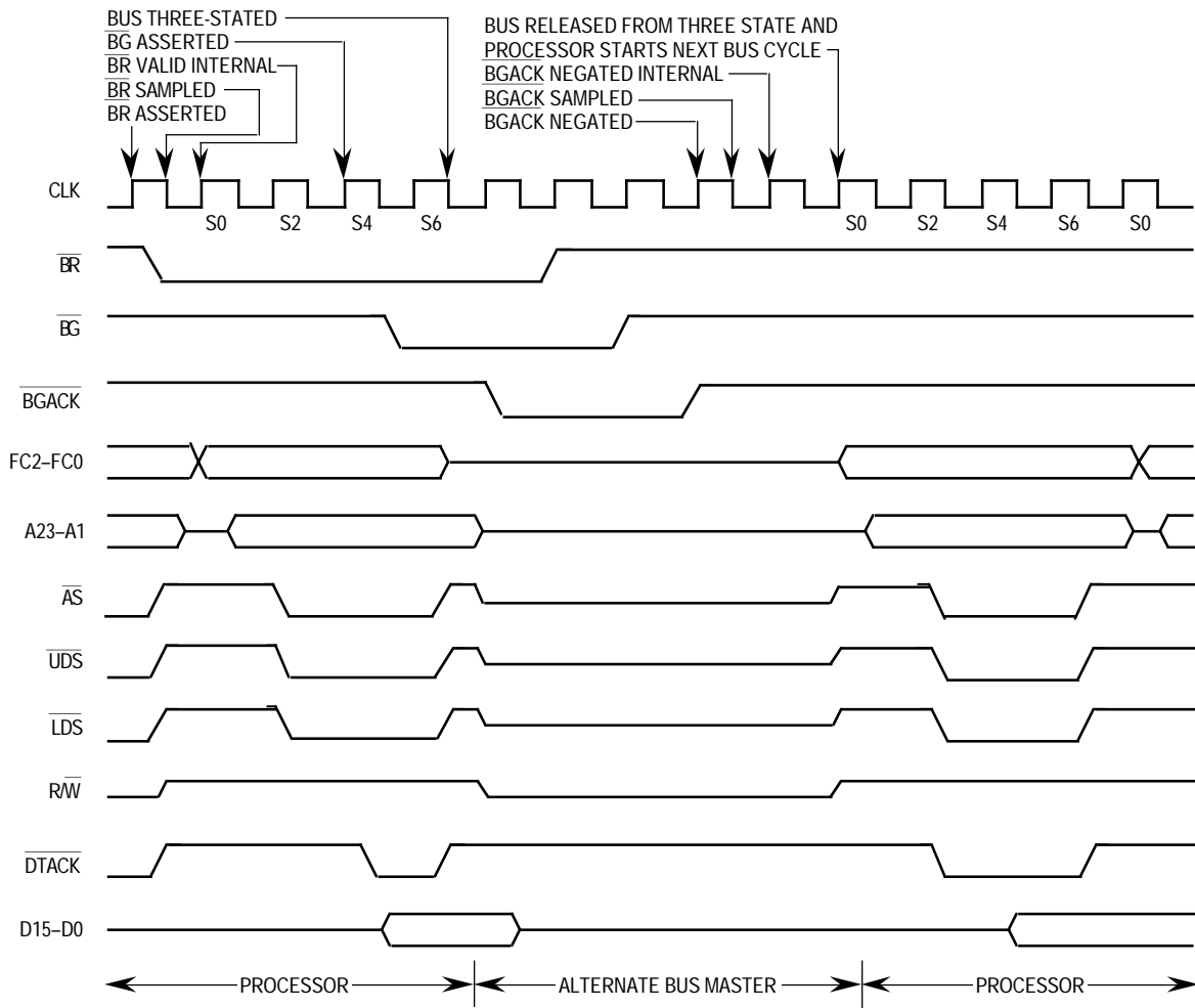
Figure 5-21. 3-Wire Bus Arbitration Timing Diagram—Special Case
