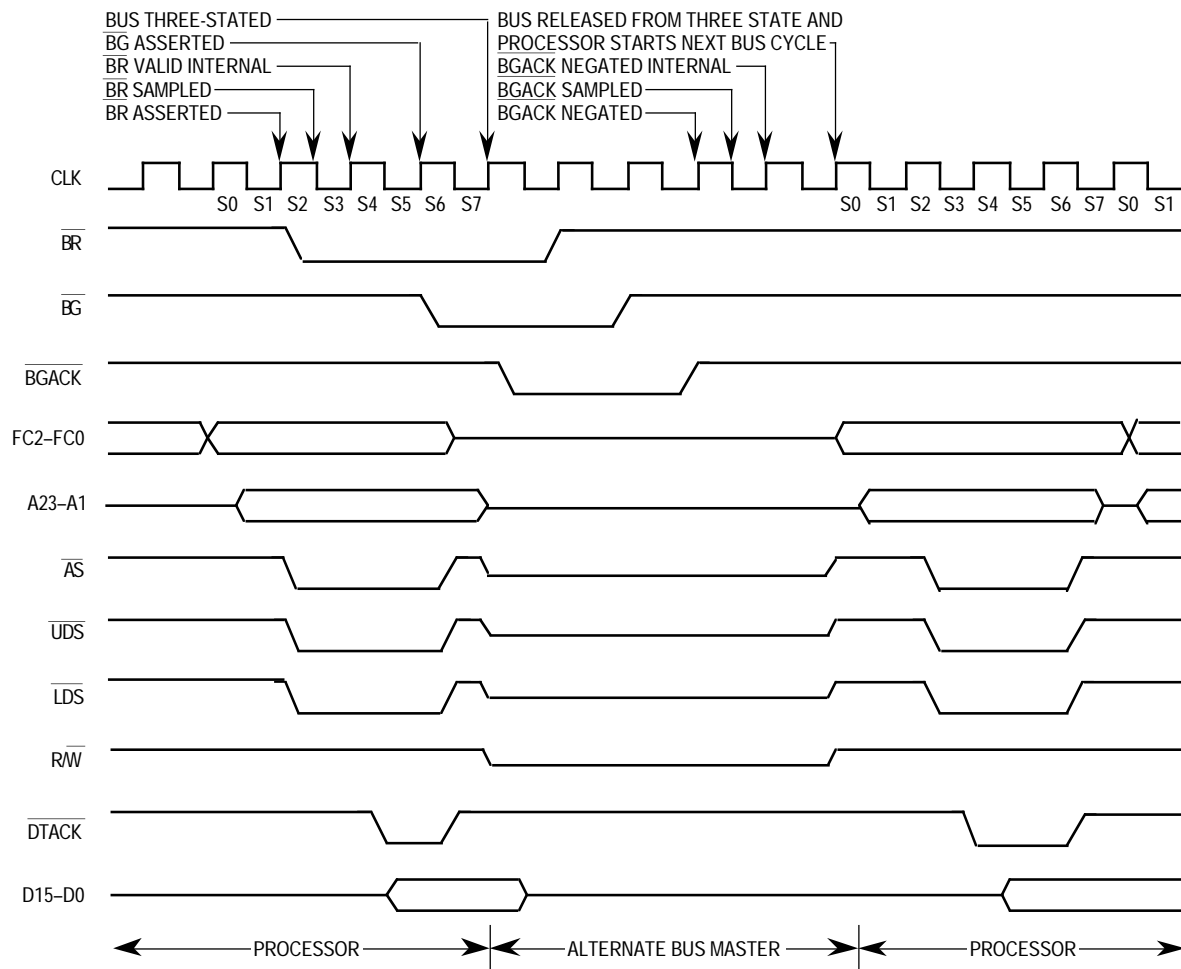
Figure 5-19. 3-Wire Bus Arbitration Timing Diagram—Processor Active
