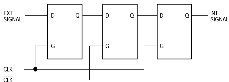
Figure 5-37. Input Synchronizers
