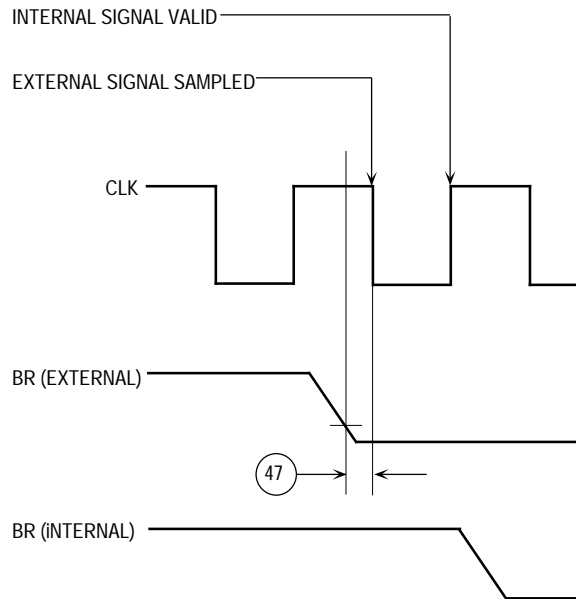
Figure 5-17. External Asynchronous Signal Synchronization
