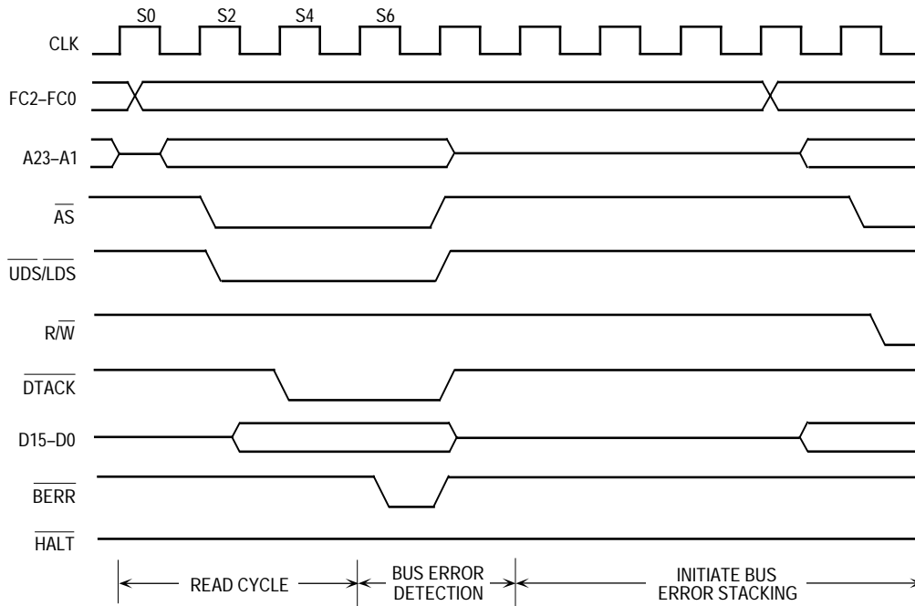
Figure 5-26. Delayed Bus Error Timing Diagram (MC68010)
