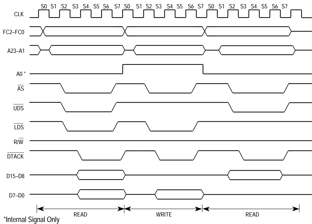
Figure 5-4. Word and Byte Read-Cycle Timing Diagram
