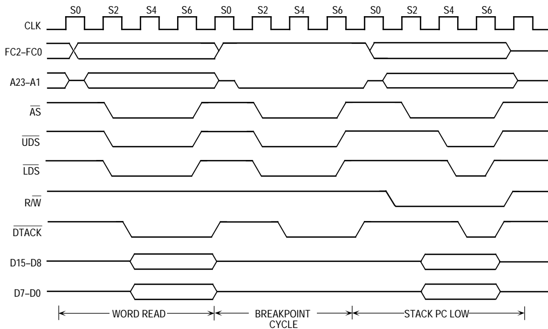
Figure 5-12. Breakpoint Acknowledge Cycle Timing Diagram
