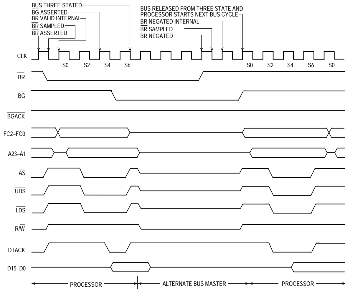
Figure 5-24. 2-Wire Bus Arbitration Timing Diagram—Special Case
