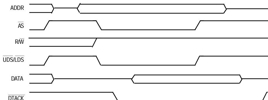
Figure 5-31. Fully Asynchronous Read Cycle
