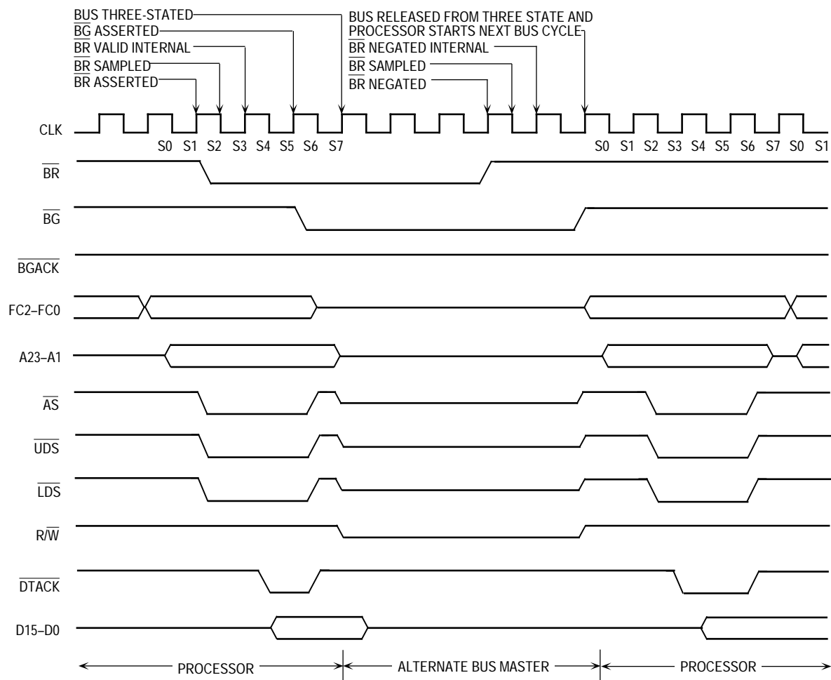
Figure 5-22. 2-Wire Bus Arbitration Timing Diagram—Processor Active
