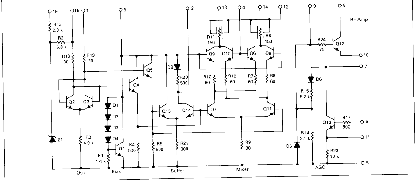
FIGURE 2 — INTERNAL SCHEMATIC
