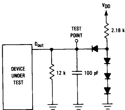
Figure 7. Test Circuit
