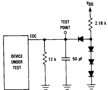
Figure 8. Test Circuit
