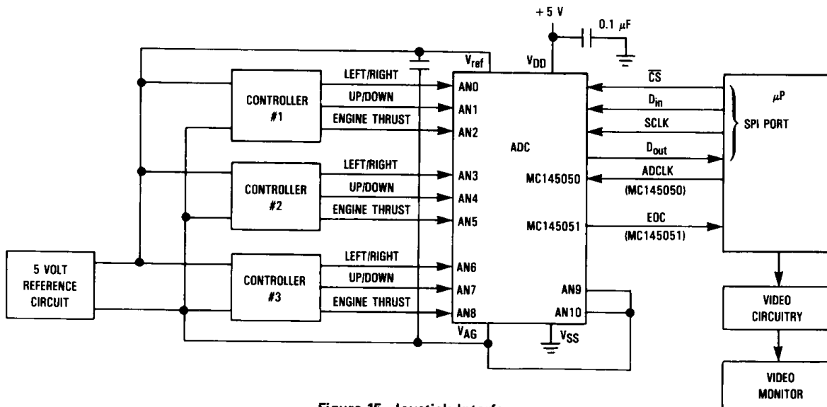
Figure 15. Joystick Interface
