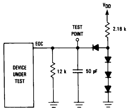
Figure 8. Test Circuit
