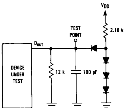
Figure 7. Test Circuit
