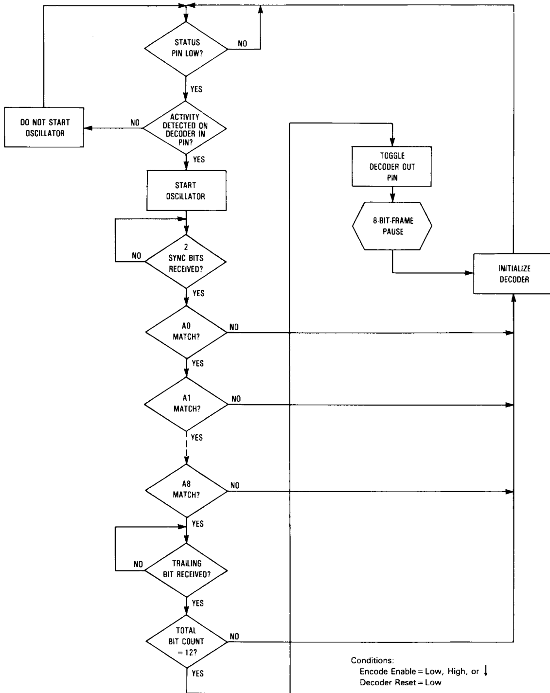
Figure 7. Decoder Flowchart
