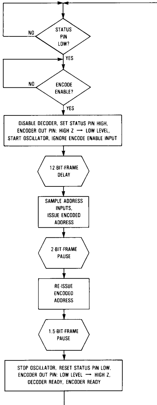
Figure 8. Encoder Flowchart
