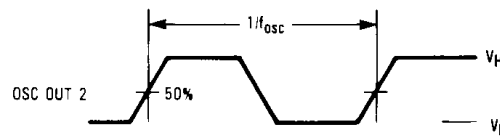
Figure 2. Switching Waveform
