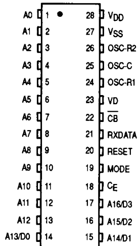
MC145032 DECODER
