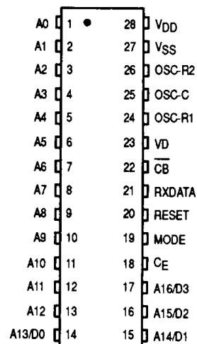
MC145035 DECODER
