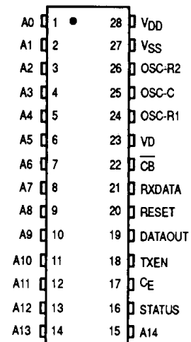
MC145033 ENCODER/DECODER
