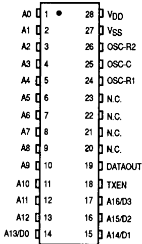
MC145031 ENCODER
