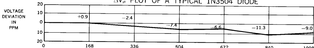
FIGURE 4 — OPERATING TEST TIME IN HOURS
