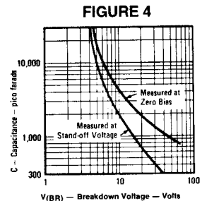
FIGURE 4 Typical Capacitance vs. Breakdown Voltage (Bidirectional Types)
