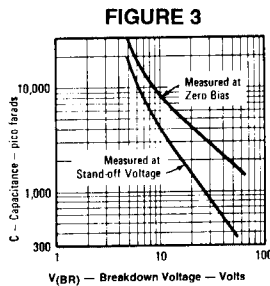
FIGURE 3 Typical Capacitance vs. Breakdown Voltage (Unidirectional Types)
