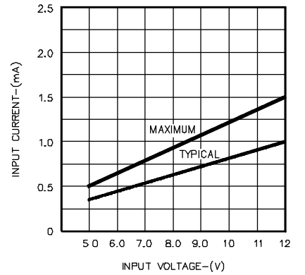
FIGURE 6. INPUT CHARACTERISTICS - SG2804
