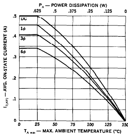
6. Average Current vs. Ambient Temperature
