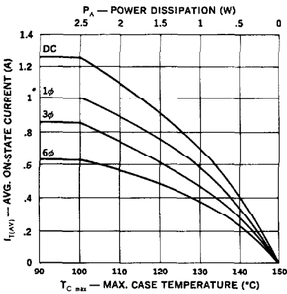
5. Average Current vs. Case Temperature
