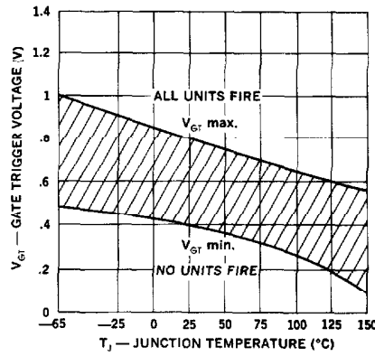
2. Gate Trigger Voltage
