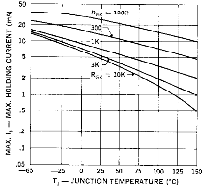
2. Max. Holding Current (Resistor Bias)
