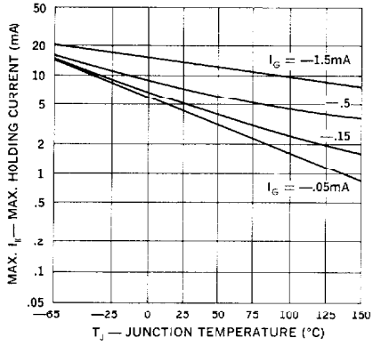
1. Max. Holding Current (Current Bias)
