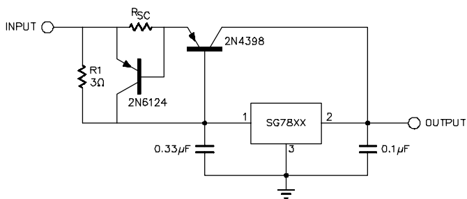
FIGURE 7 - HIGH OUTPUT CURRENT, SHORT CIRCUIT PROTECTED
