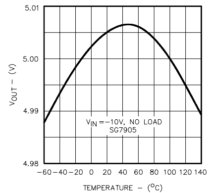
FIGURE 3. TEMPERATURE COEFFICIENT
