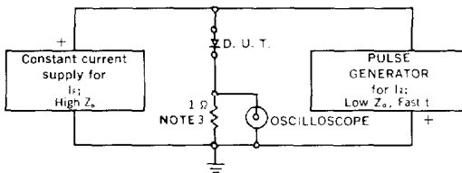
Reverse-Recovery Circuit
