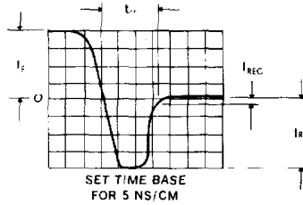
Characteristic Waveform
