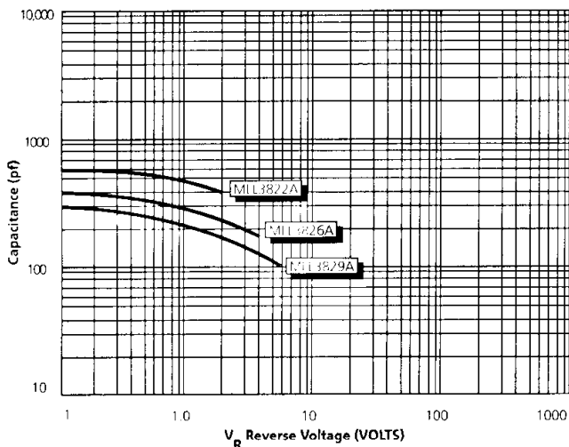
FIGURE 4 Typical Capacitance vs. Reverse Voltage
