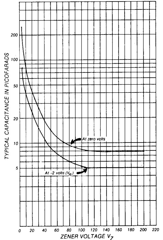
CAPACITANCE vs. V_Z CURVE
