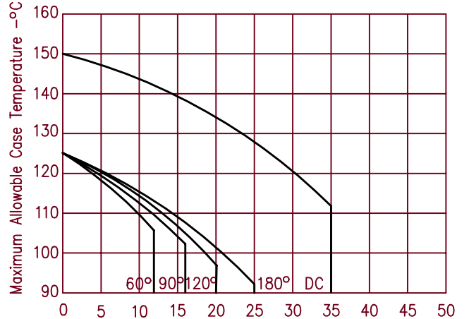
Figure 5 Forward Current Derating - Reverse Polarity
