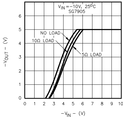
FIGURE 7. DROPOUT CHARACTERISTICS
