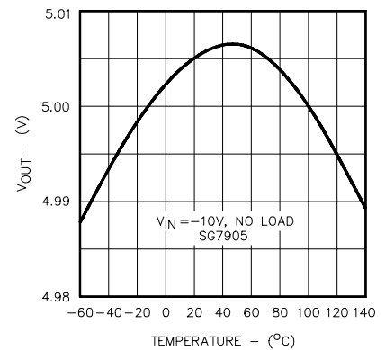
FIGURE 3. TEMPERATURE COEFFICIENT
