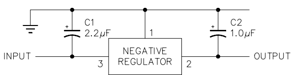
FIGURE 9 - FIXED OUTPUT REGULATOR
