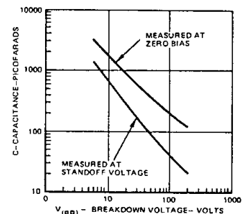
FIGURE 4 TYPICAL CAPACITANCE VS. BREAKDOWN VOLTAGE
