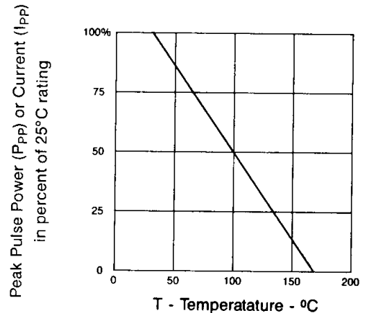
FIGURE 3 DERATING CURVE
