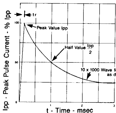
FIGURE 2 PULSE WAVEFORM
