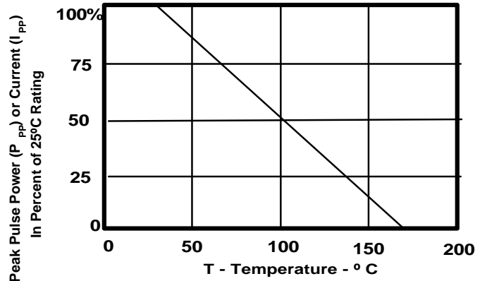
FIGURE 3 Derating Curve
