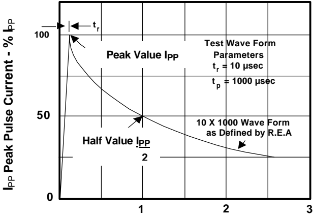
t - Time - msec Figure 2 Pulse Waveform
