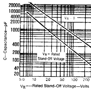
FIGURE 4 TYPICAL CAPACITANCE VS STAND-OFF VOLTAGE
