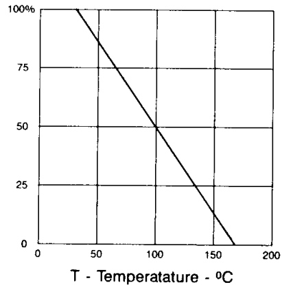
FIGURE 3 DERATING CURVE
