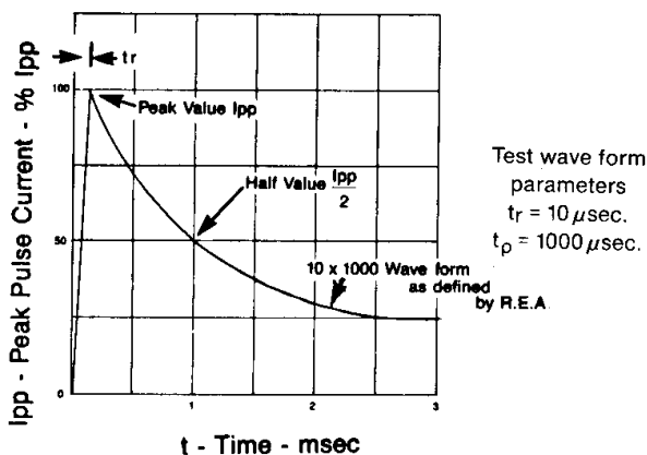
FIGURE 2 PULSE WAVEFORM
