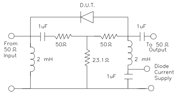
TEST CIRCUIT FOR DISTORTION MEASUREMENTS
