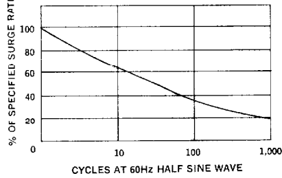
Multiple Forward Surge Rating
