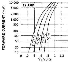
Typical Forward Voltage vs Forward Current
