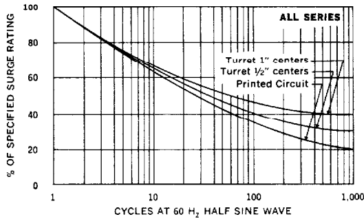
Allowable Forward Surge vs Number of Cycles
