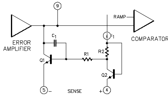
FIGURE 3 - CURRENT LIMITING CIRCUITRY OF THE SG1524
