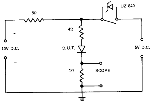
Reverse Recovery Circuit
