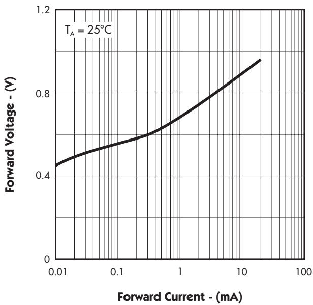
FIGURE 3. — FORWARD CHARACTERISTICS
