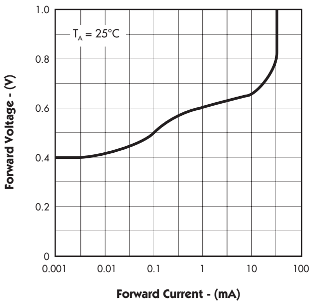
FIGURE 10. — FORWARD CHARACTERISTICS
