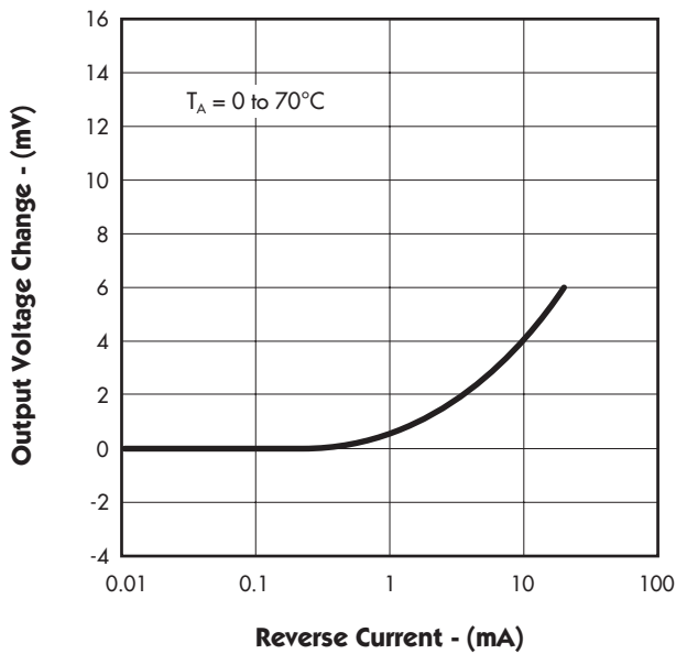
FIGURE 5. — REVERSE VOLTAGE CHANGE
