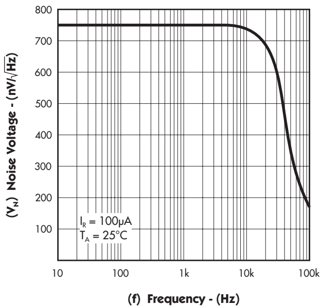
FIGURE 7. — NOISE VOLTAGE
