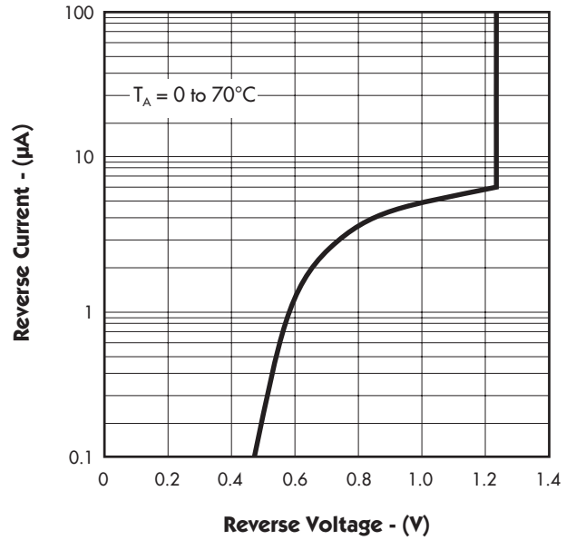
FIGURE 2. — REVERSE CHARACTERISTICS
