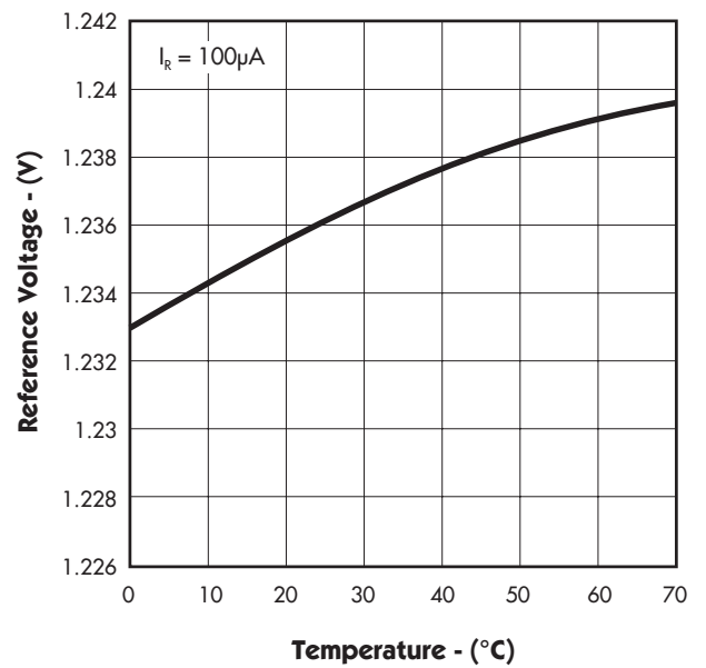
FIGURE 4. — TEMPERATURE DRIFT
