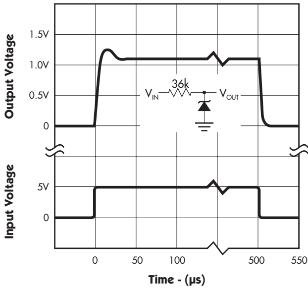
FIGURE 1. — RESPONSE TIME
