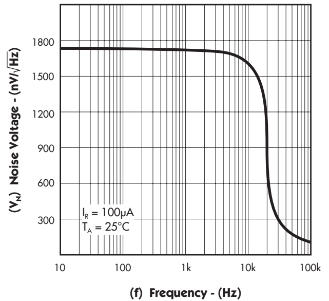
FIGURE 13. — NOISE VOLTAGE
