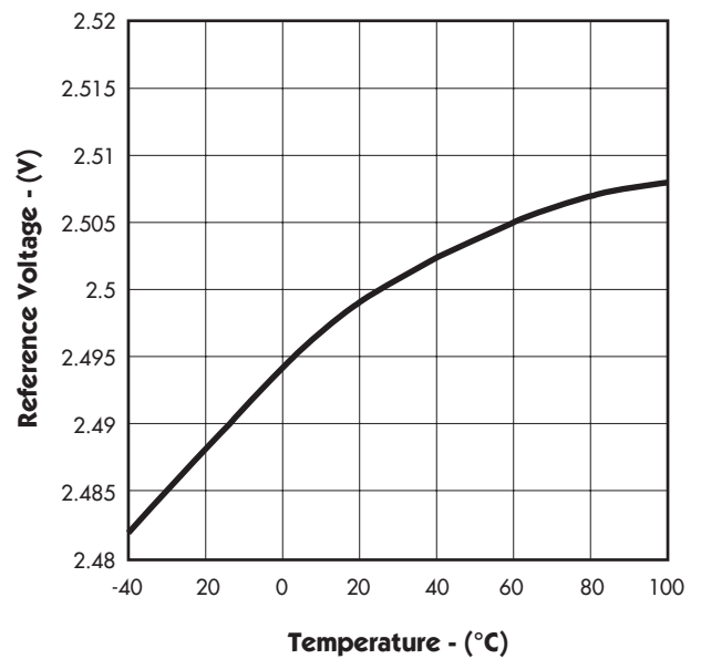
FIGURE 11. — TEMPERATURE DRIFT
