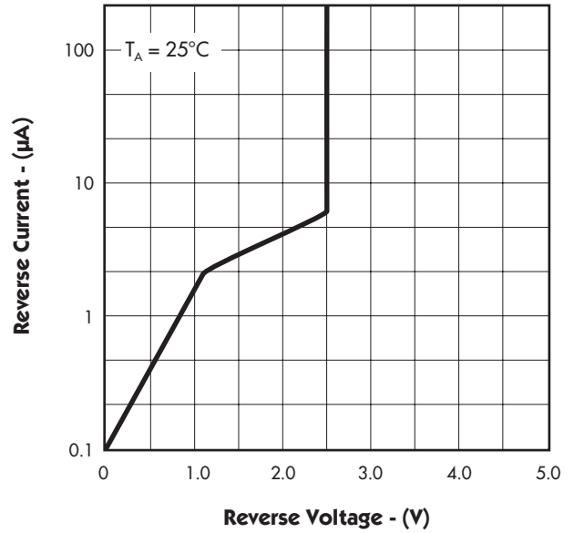
FIGURE 9. — REVERSE CHARACTERISTICS
