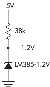
1.2V REFERENCE
