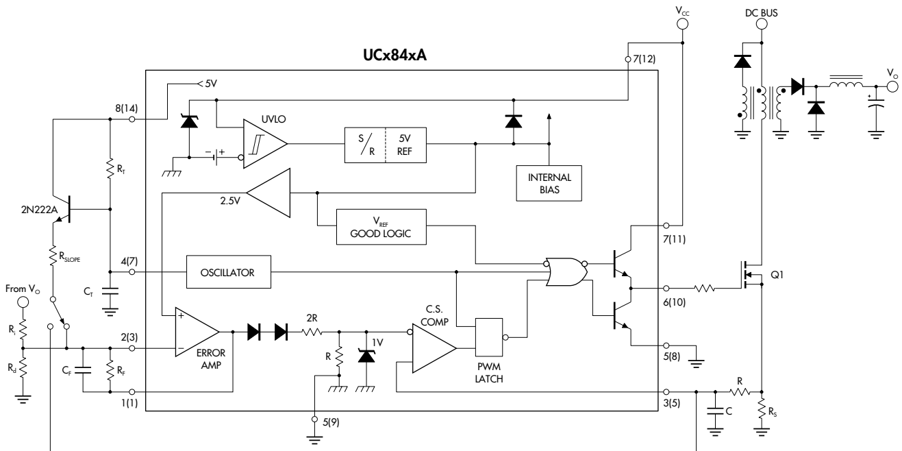
FIGURE 6. — SLOPE COMPENSATION
